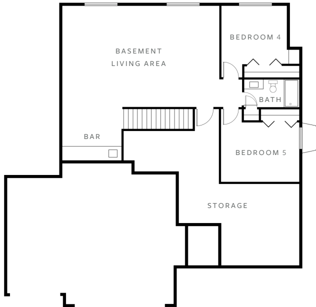
BASEMENT (960 SF OPTIONAL)
